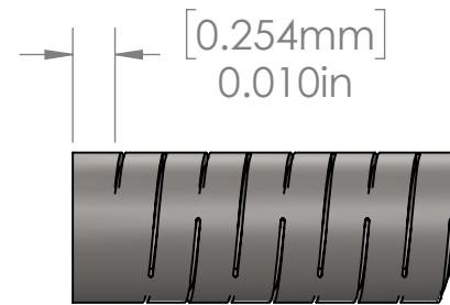
DETAIL A SCALE 20 : 1
