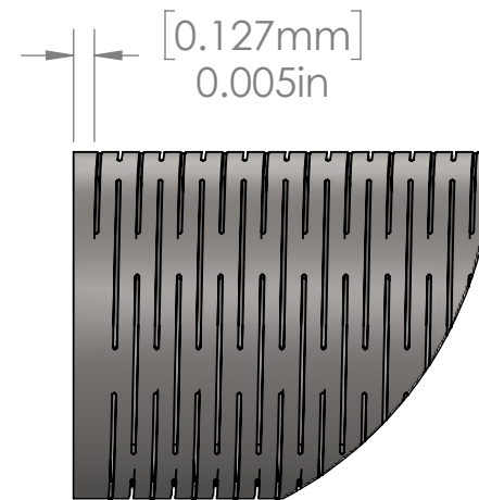
DETAIL A SCALE 20 : 1
