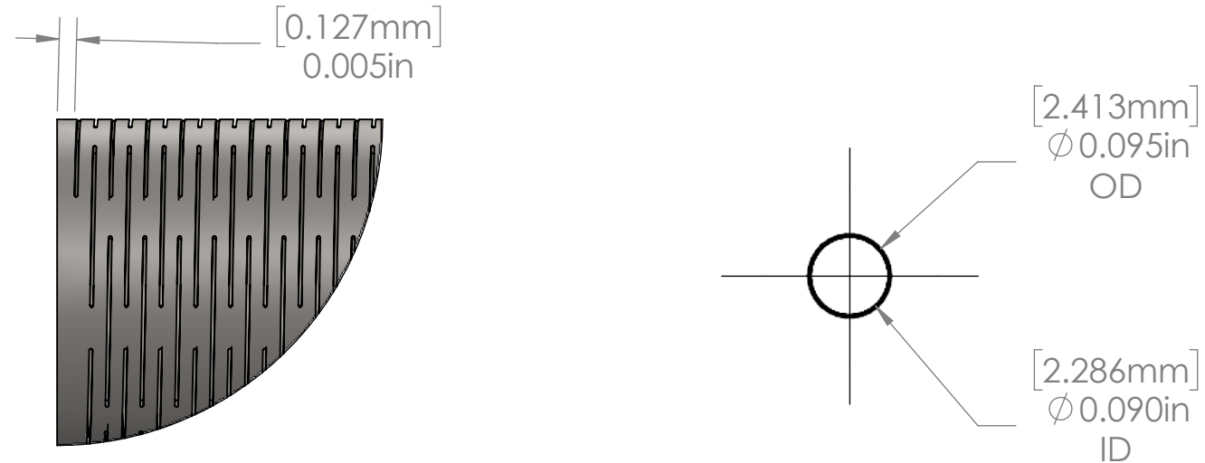
DETAIL A SCALE 20 : 1
